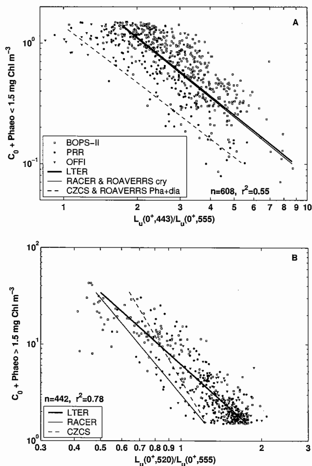
Figure 7. Water-leaving radiance ratios used in the CZCS general processing algorithm: (a) the ratio of L_u(443)/L_u(555) for chlorophyll and phaeopigment concentrations < 1.5 \text{ mg Chl m}^{-3} and (b) the ratio L_u(520)/L_u(555) for chlorophyll concentrations > 1.5 \text{ mg Chl m}^{-3} . The thick solid lines are the best fit lines for all LTER data, and the dashed lines represent the general processing CZCS algorithms [Gordon and Morel, 1983]. The RACER data are from Antarctic Peninsula waters [Mitchell and Holm-Hansen, 1991]. The Research on Ocean-Atmosphere Variability and Ecosystem Response in the Ross Sea (ROAVERRS) data are from the Ross Sea [Arrigo et al., 1998], where cryp is cryptophytes, Pha is Phaeocystis Antarctica , and dia is diatoms.
