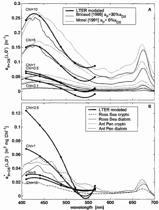
Figure 9. (a) Absorption due to particulates and dissolved organic matter a_{P+DS}(\lambda, 0^-) , estimated from the BOPS-II data using Gershun's law (equation (10)) and subtracting a_w [Pope and Fry, 1997]. Modeled estimates of a_{P+DS}(\lambda, 0^-) from Bricaud et al. [1995] and Morel [1991]. Mean standard deviation is \pm 0.032 . (b) Pigment-specific absorption a_{P+DS}^*(\lambda, 0^-) for different chlorophyll concentrations. Ross Sea data are from Arrigo et al. [1998], and Antarctic Peninsula data are from Brody et al. [1992].
